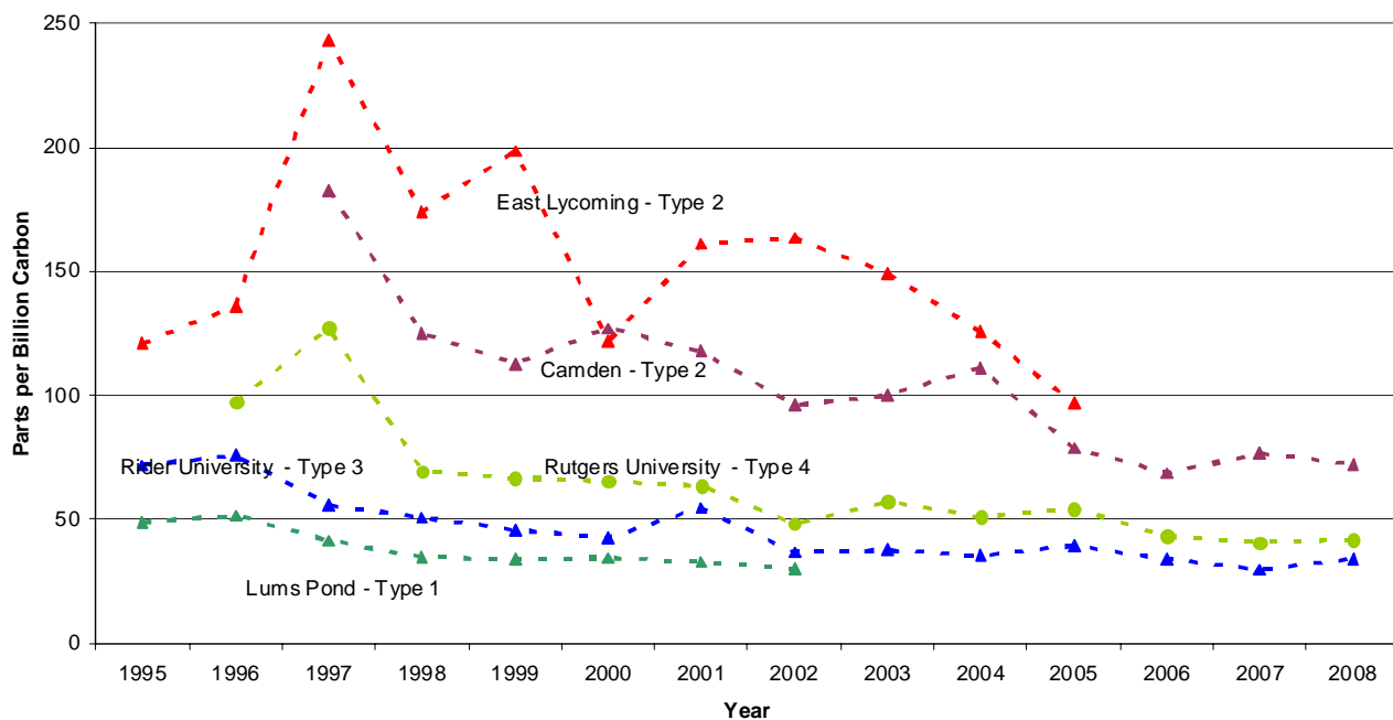
Figure 3 Philadelphia Region Total Non-methane Organic Carbon (TNMOC) Seasonal Average 1995-2008
