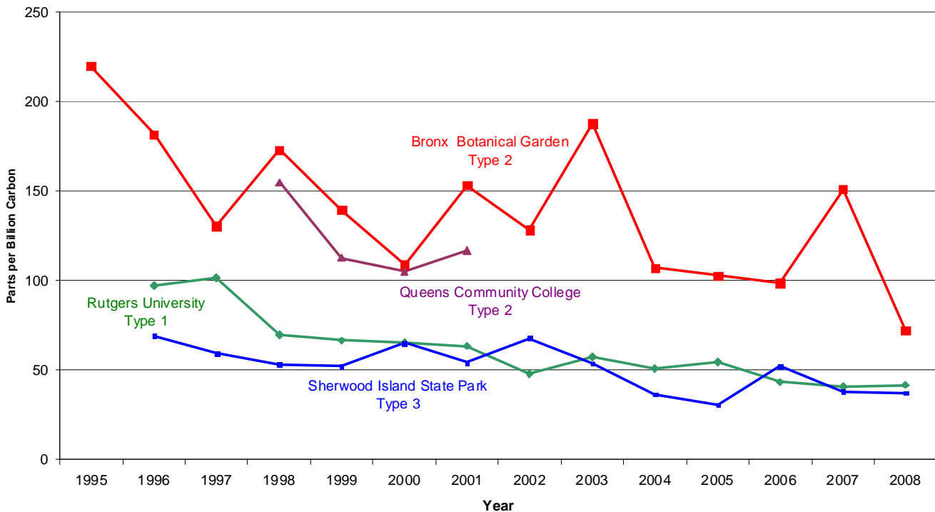
Figure 4 New York City Region Total Non-methane Organic Carbon (TNMOC) Seasonal Average 1995-2008
